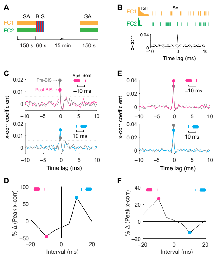
Fig. 1. STDP regulates synchrony in fusiform cells of the guinea pig DCN.
